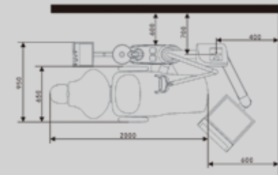
Exteranal floor-box installation sketch map
