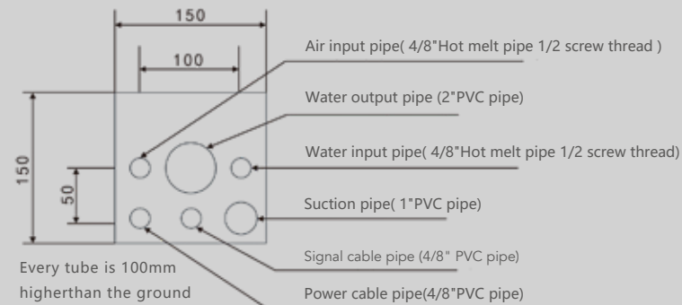
Pre-buried pipe distribution map
